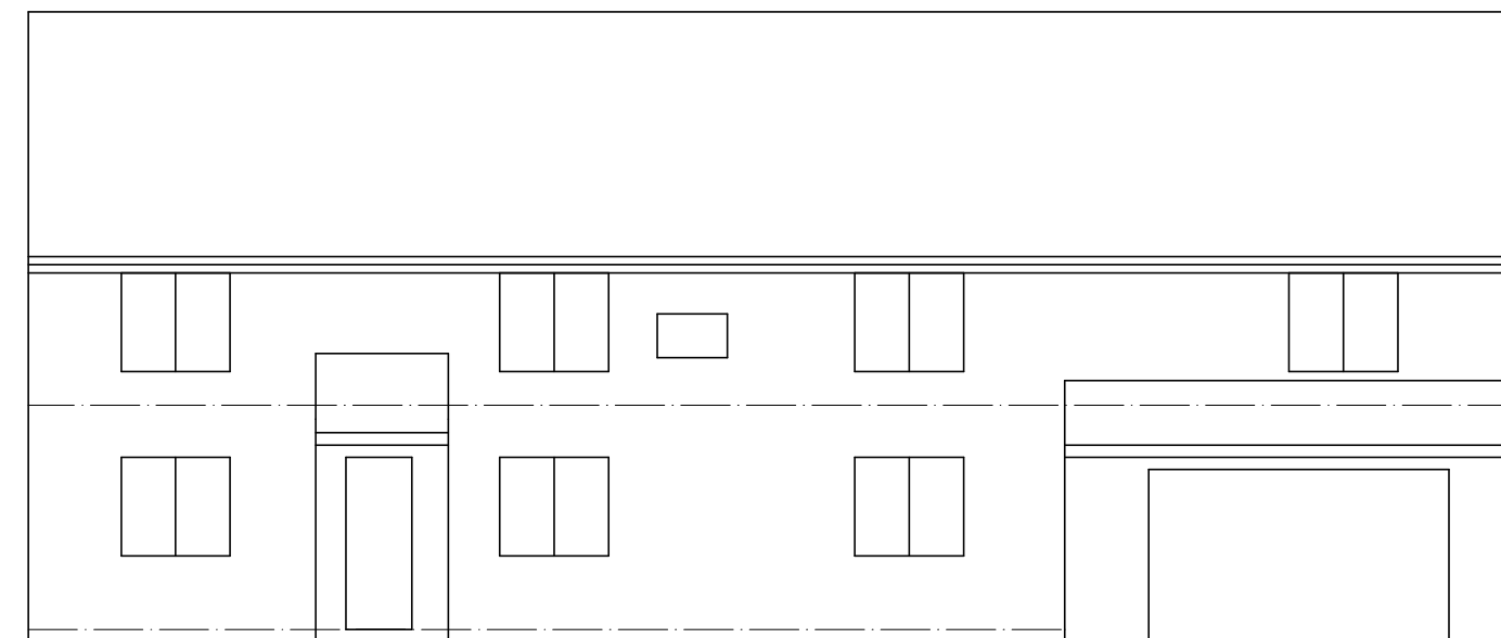
FRONT ELEVATION
