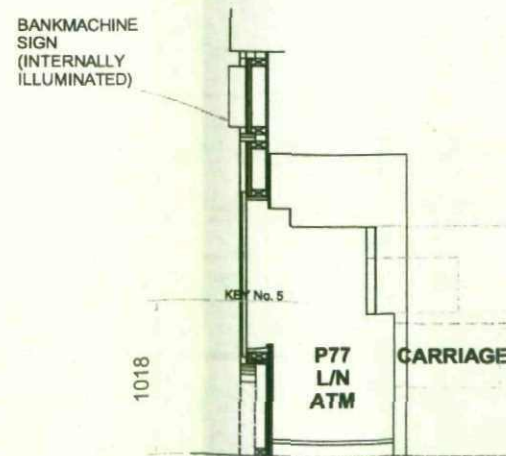
SECTION AT ATM LOCATION 1:50
