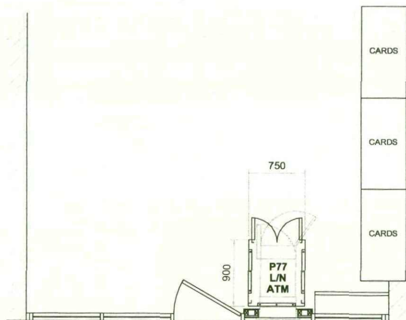
PROPOSED (PART) PLAN 1:50
