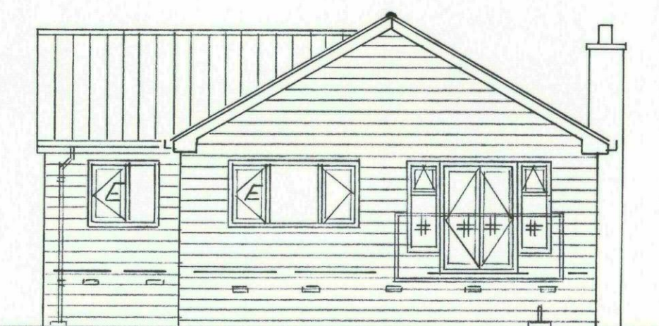
PROPOSED REAR
