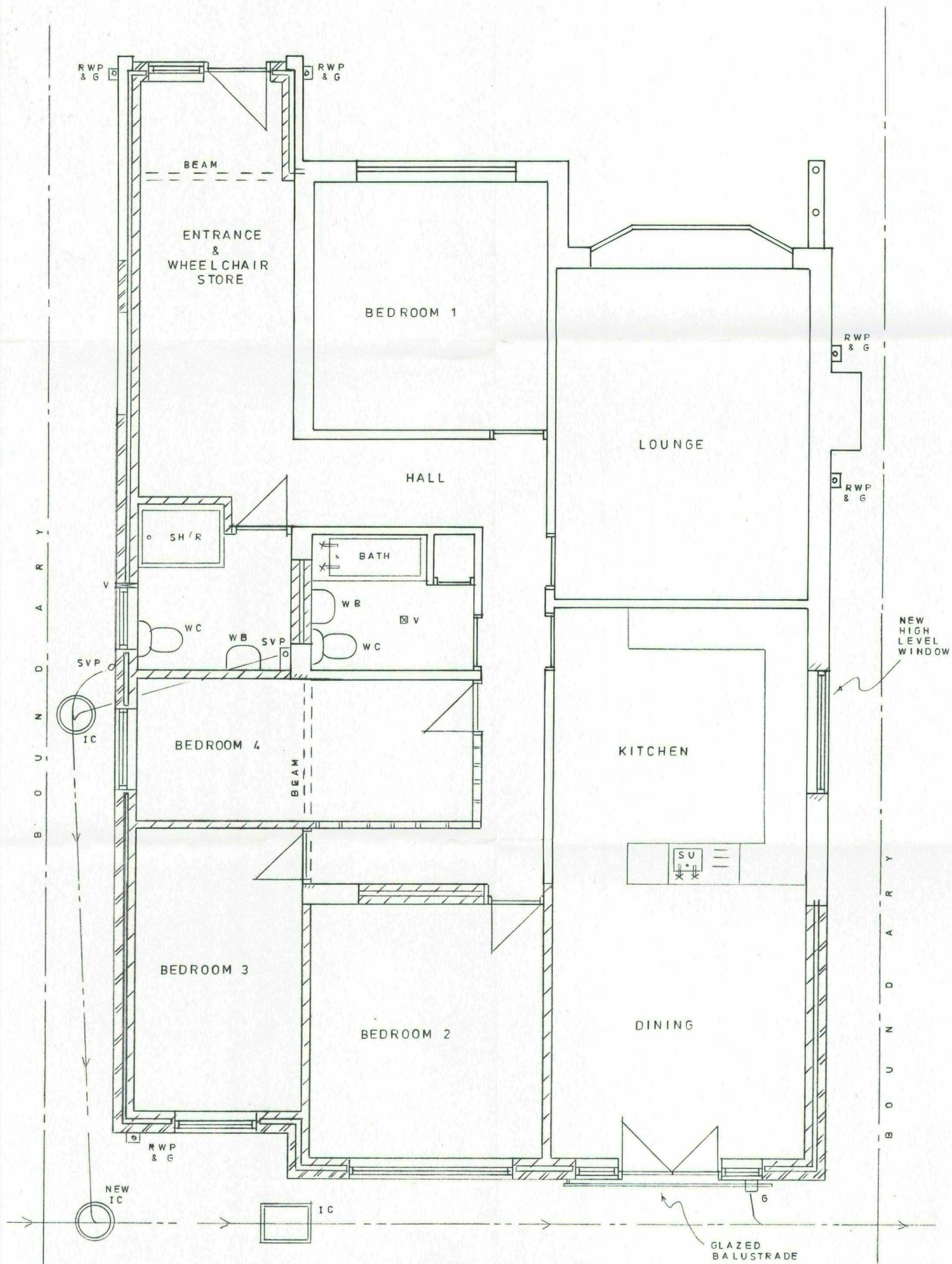
PROPOSED PLAN
