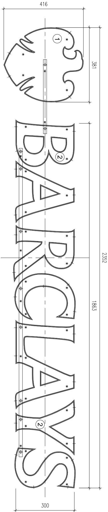
STANDARD INDIVIDUAL LETTER LOGO CONFIGURATION Scale 1:10
