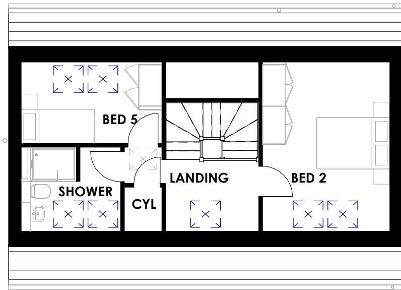
SECOND FLOOR 1 : 100
