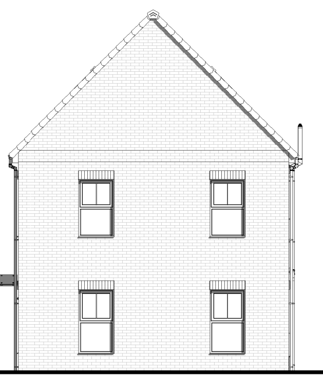
SIDE ELEVATION 1 : 100
