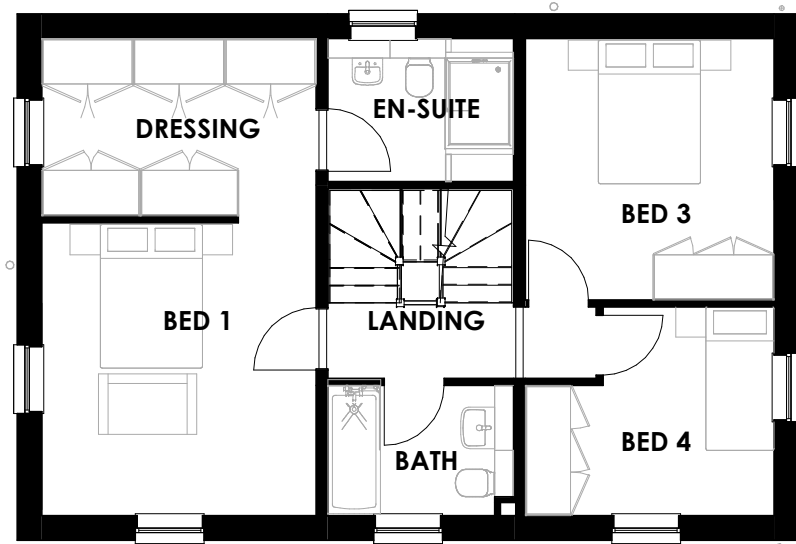
FIRST FLOOR 1 : 100
