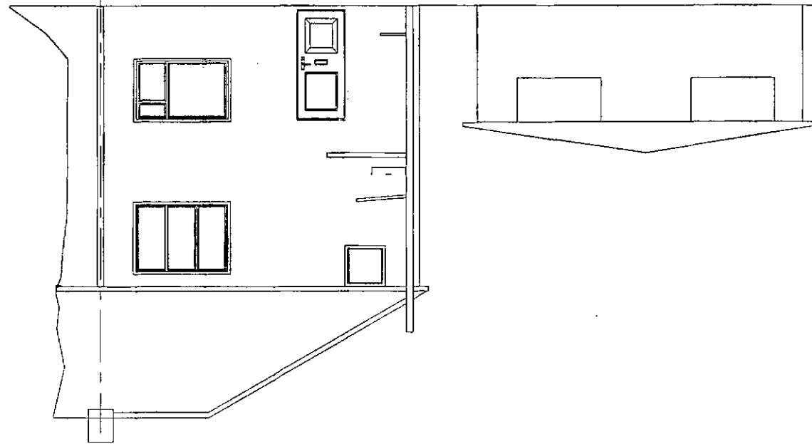
EXISTING REAR MINUS CONSERVATORY ELEVATION 1:100
