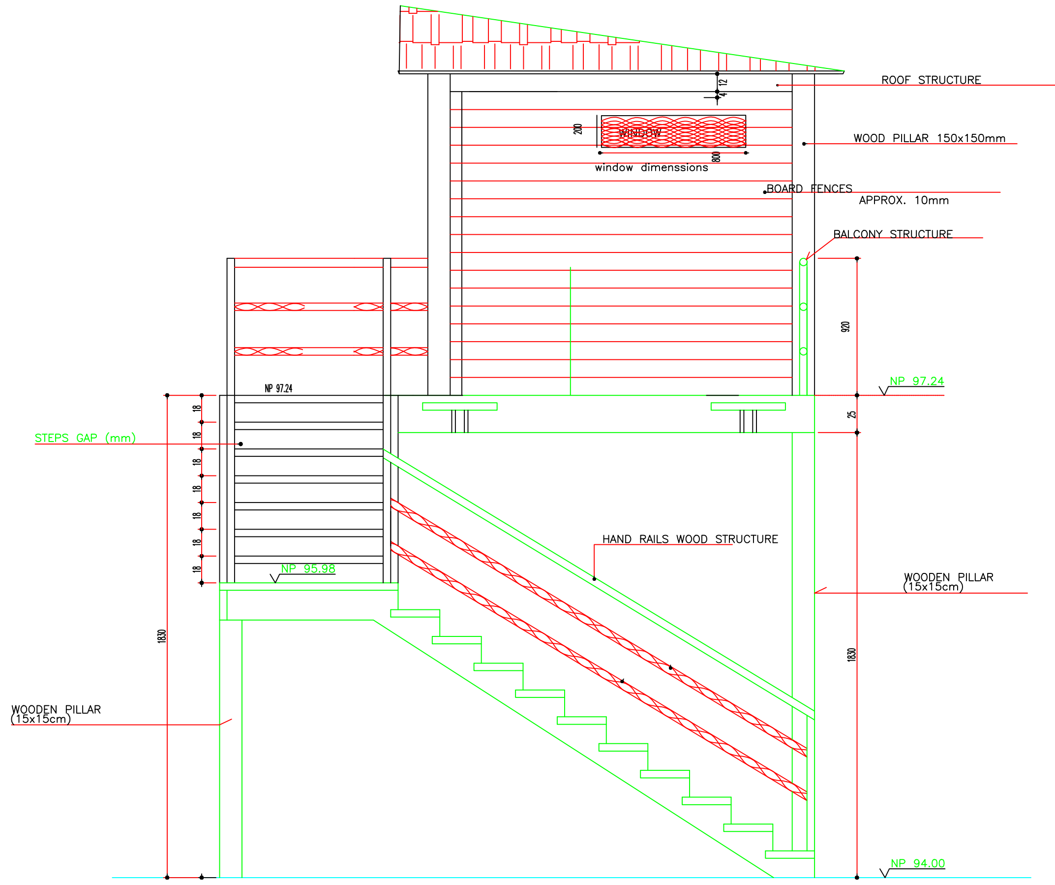
Drawing.4 – Elevation "D" – SIDE View SCALE– 1:25
