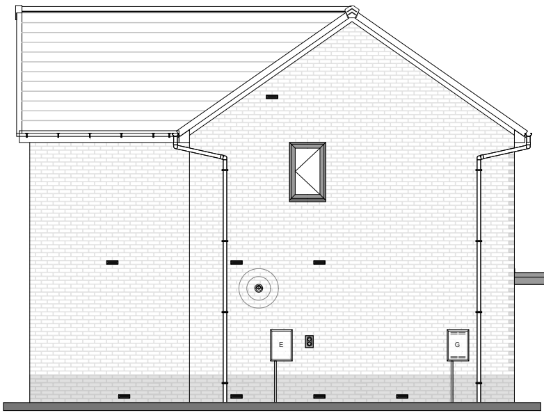
LEFT ELEVATION
