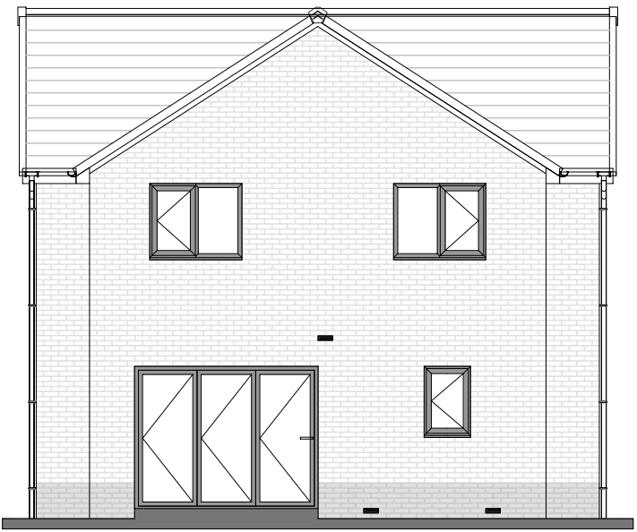
REAR ELEVATION
