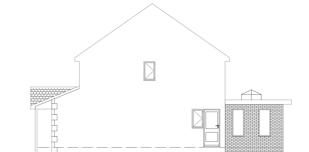
SIDE ELEVATION
