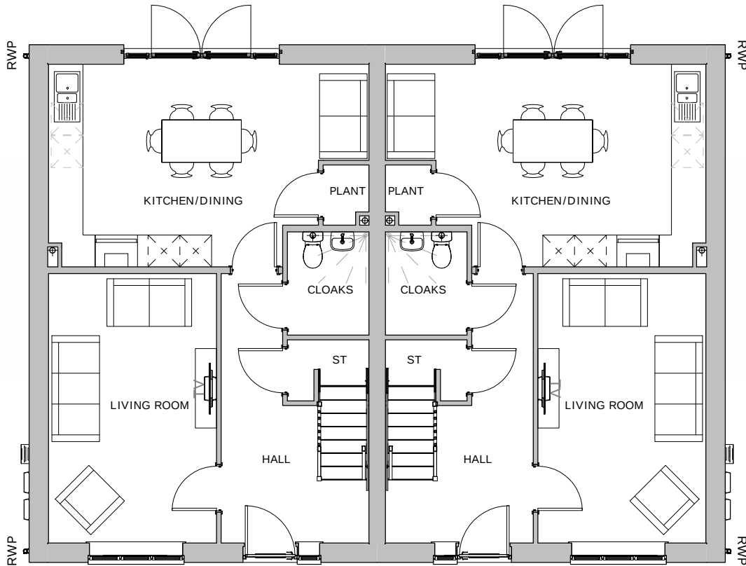
Ground Floor 1 : 100
