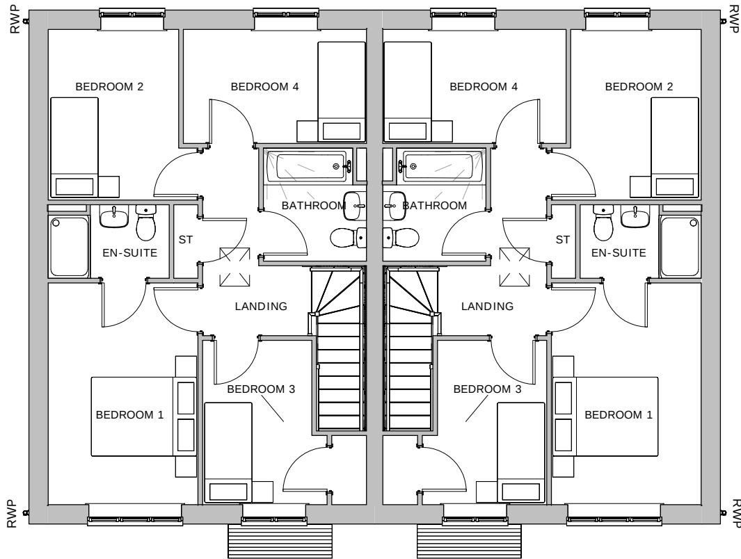
First Floor 1 : 100
