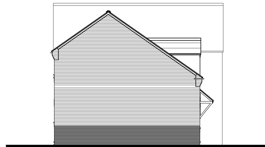
SIDE ELEVATION
