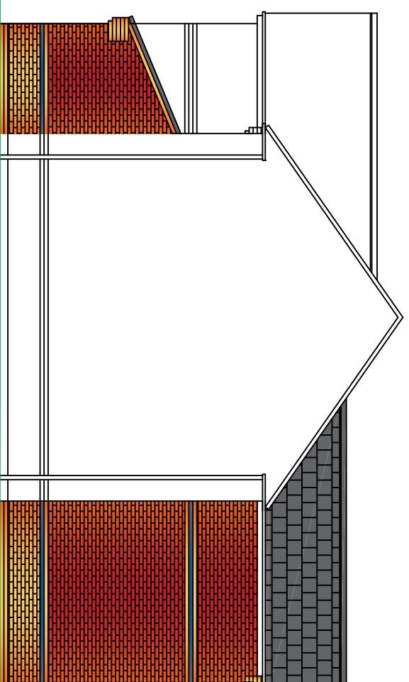
Side Elevation
