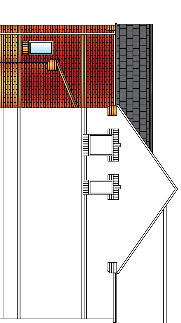
Side Elevation
