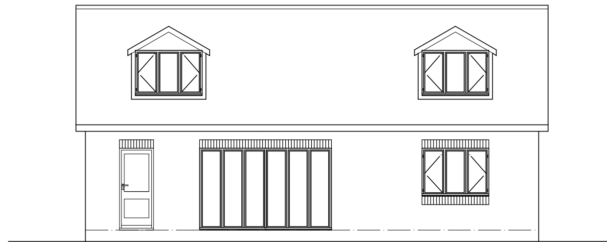
REAR ELEVATION
