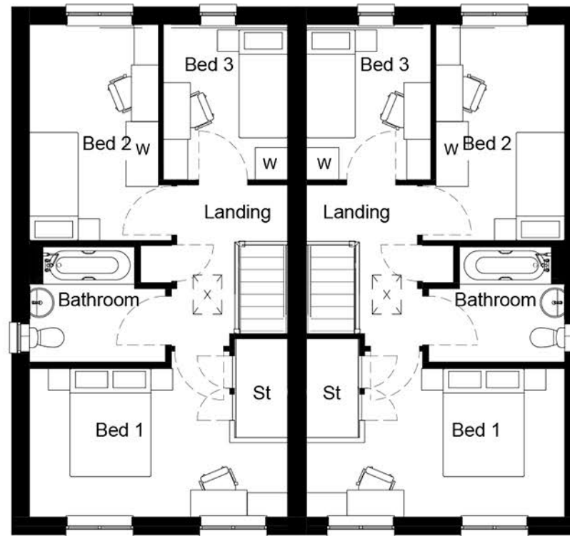
First Floor.
