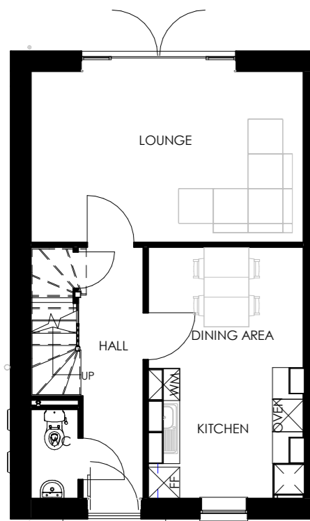
GROUND FLOOR 1 : 100
