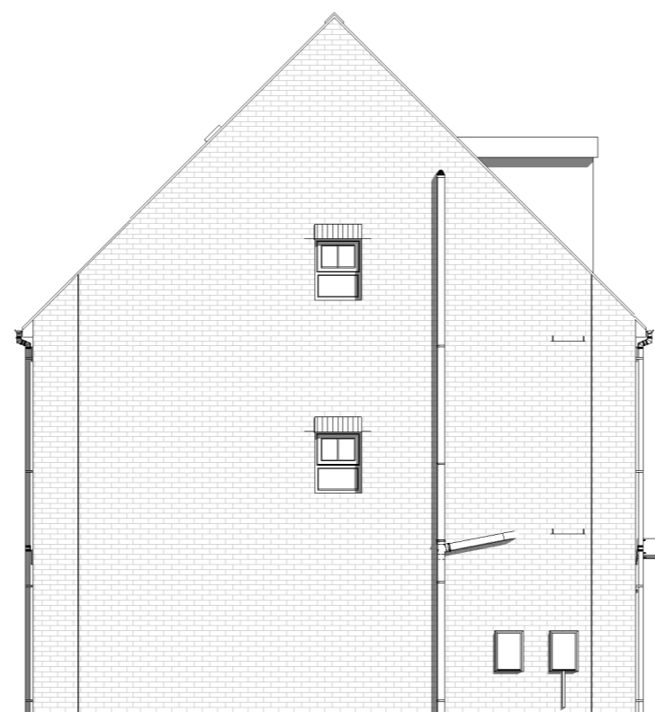
SIDE ELEVATION 1 : 100
