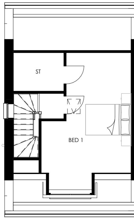
SECOND FLOOR 1 : 100
