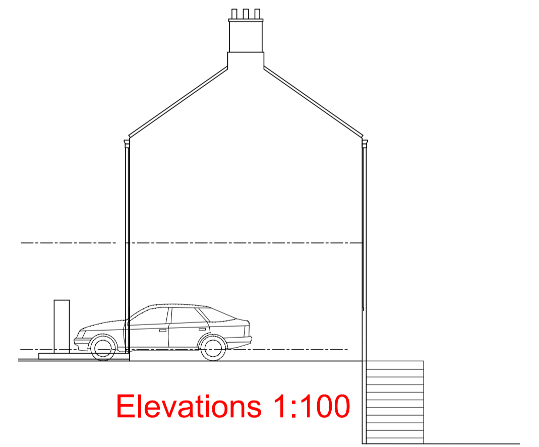
Elevations 1:100
