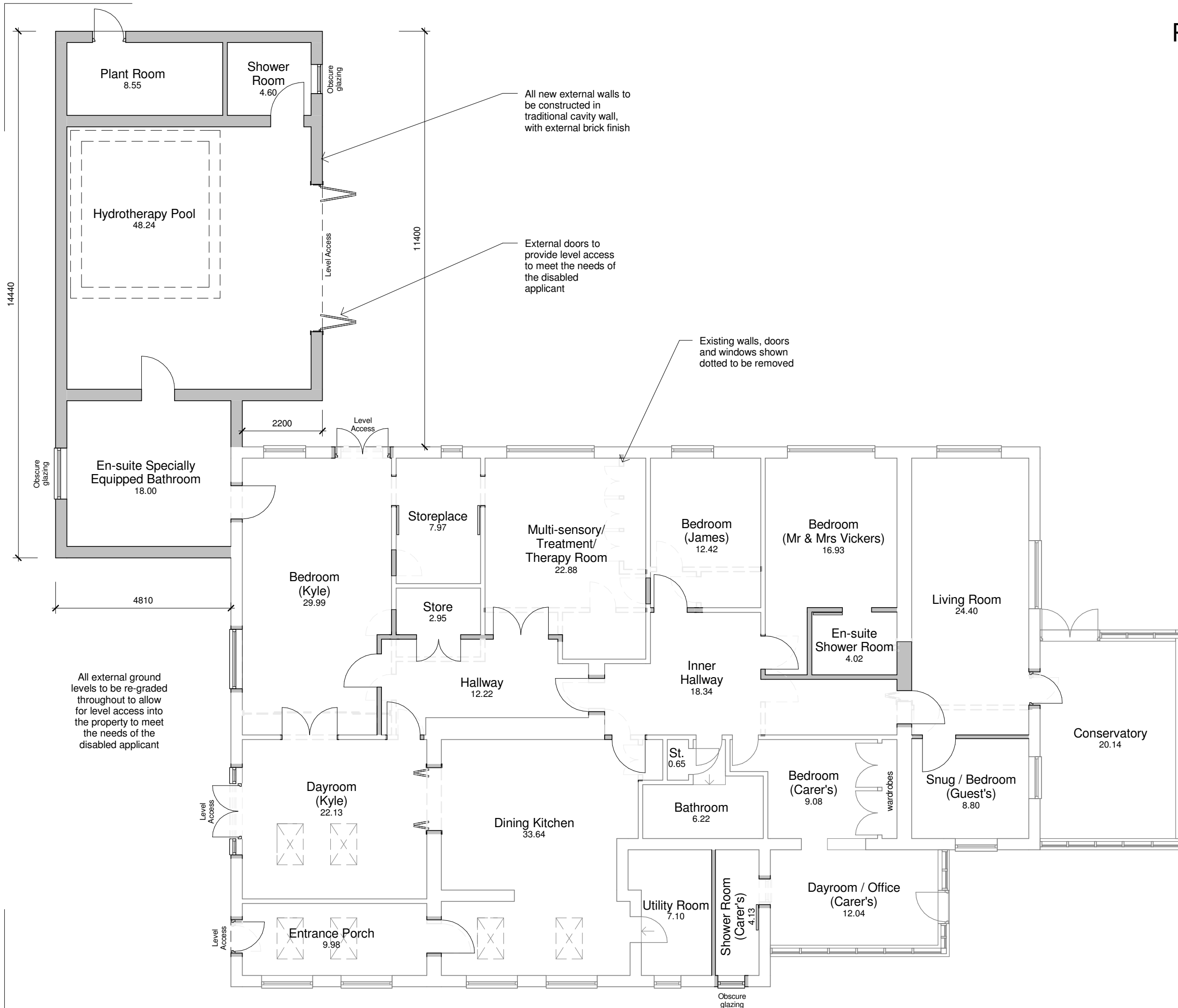
PROPOSED FLOOR LAYOUT PLAN
