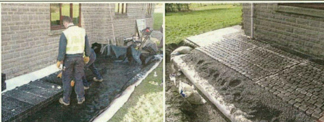
Installation of a rainwater harvester system below a permeable concrete block surface
