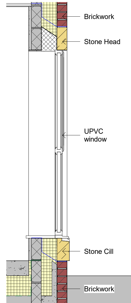
SECTION I
