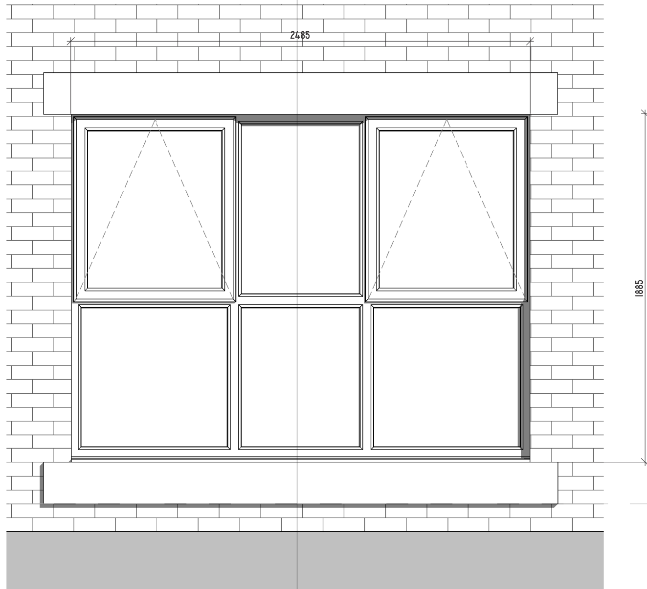
WINDOW ELEVATION
