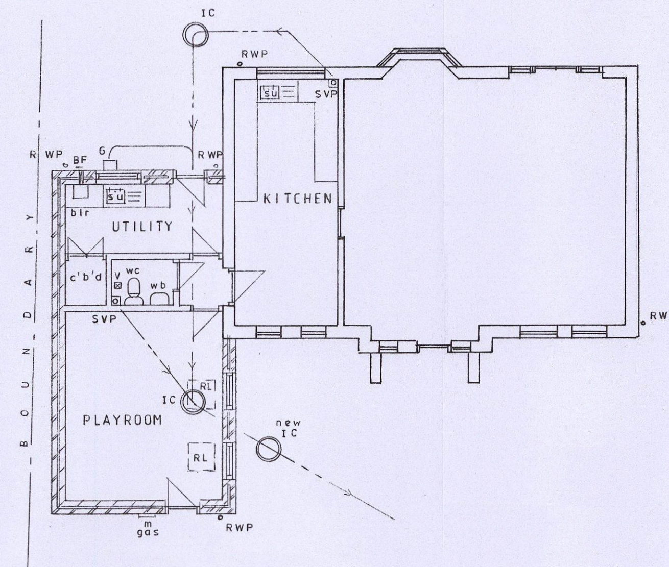
PROPOSED G.F. PLAN
