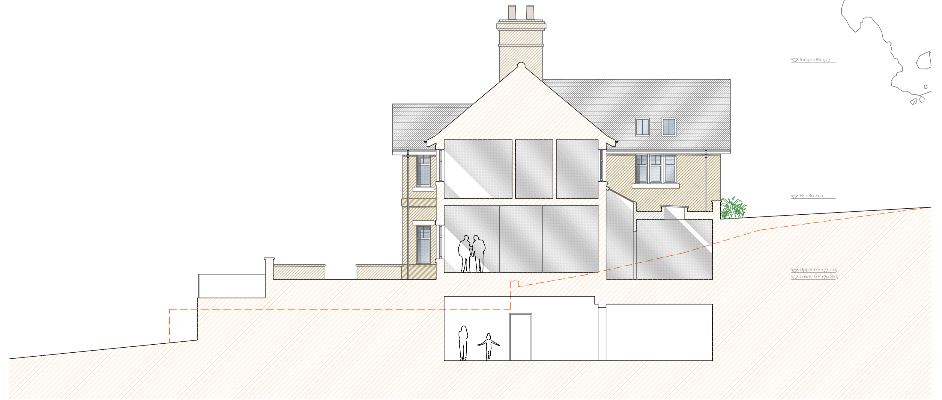
D - Building Cross Section
