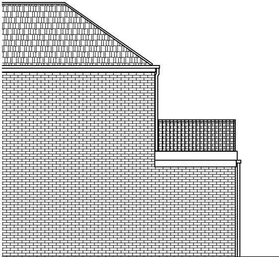
EXISTING END ELEVATION SCALE 1:100 AT A3
