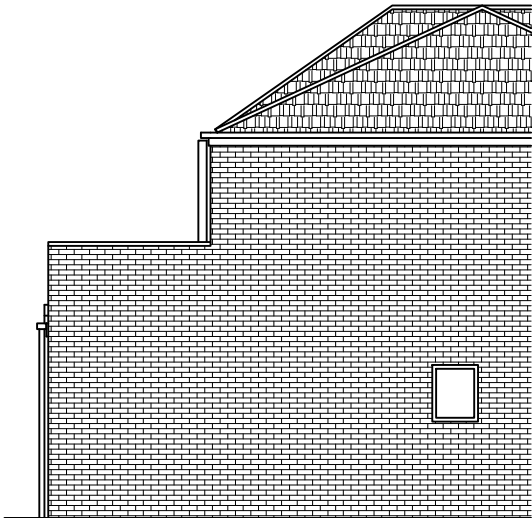
EXISTING END ELEVATION SCALE 1:100 AT A3
