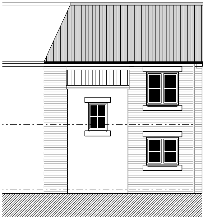
Part front elevation
