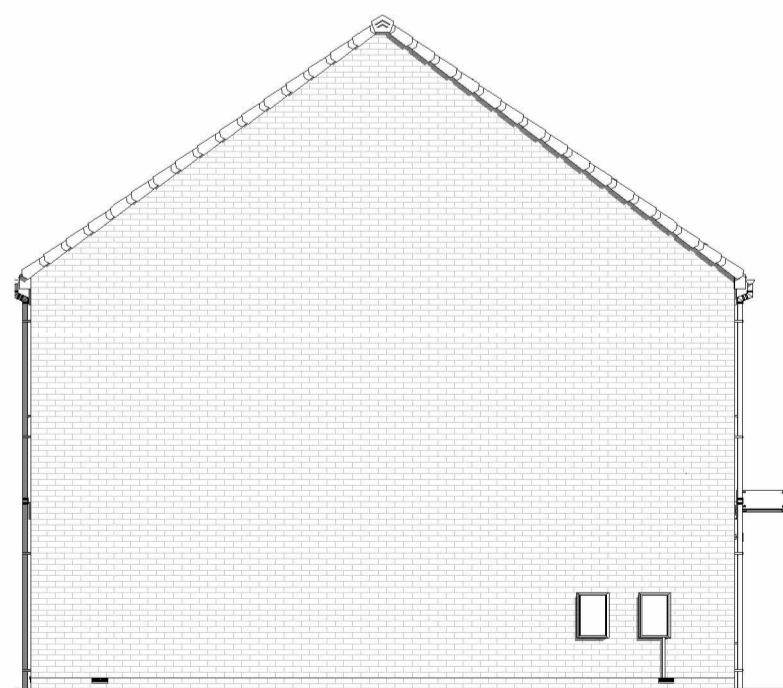
LEFT ELEVATION 1 : 100
