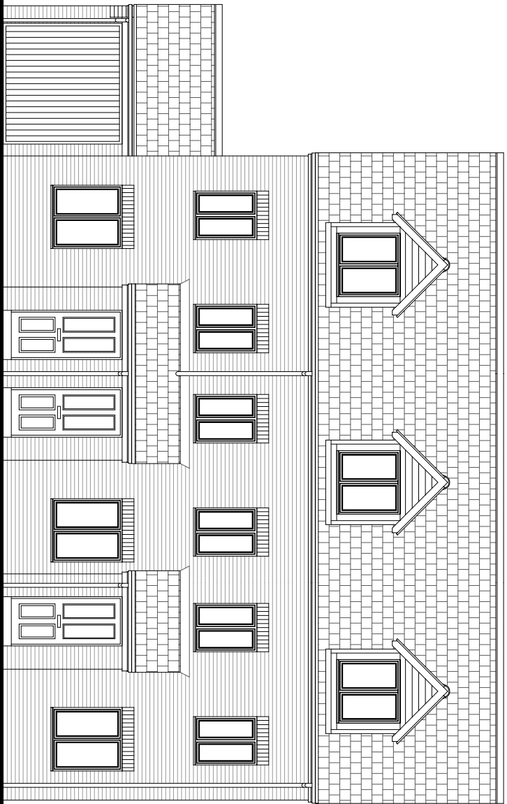
Front Elevation
