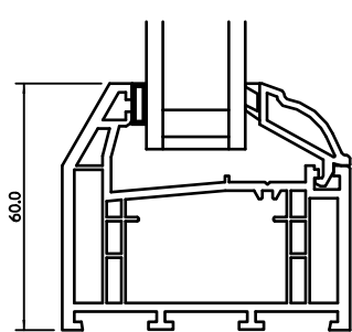
FULL SIZE SECTIONS (SSHOWN WITH 24mm GLAZING)
