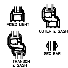
WF2, WF3 &amp; WF4 SIMILAR
