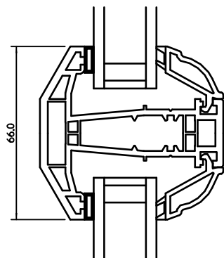
FULL SIZE SECTIONS (SSHOWN WITH 24mm GLAZING)
