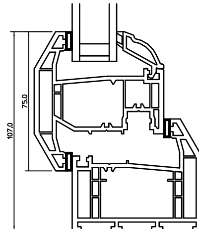
FULL SIZE SECTIONS (SSHOWN WITH 24mm GLAZING)
