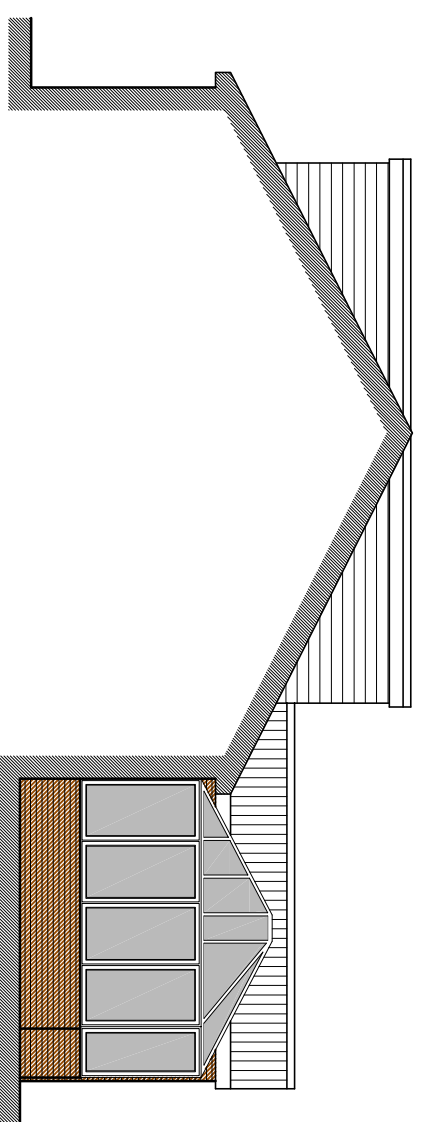
PROPOSED SIDE ELEVATION SCALE 1:100
