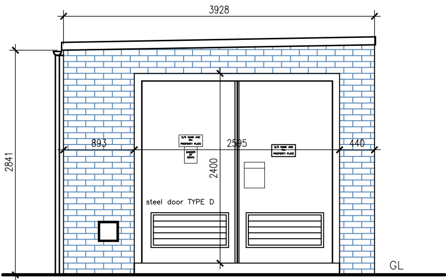
FRONT ELEVATION
