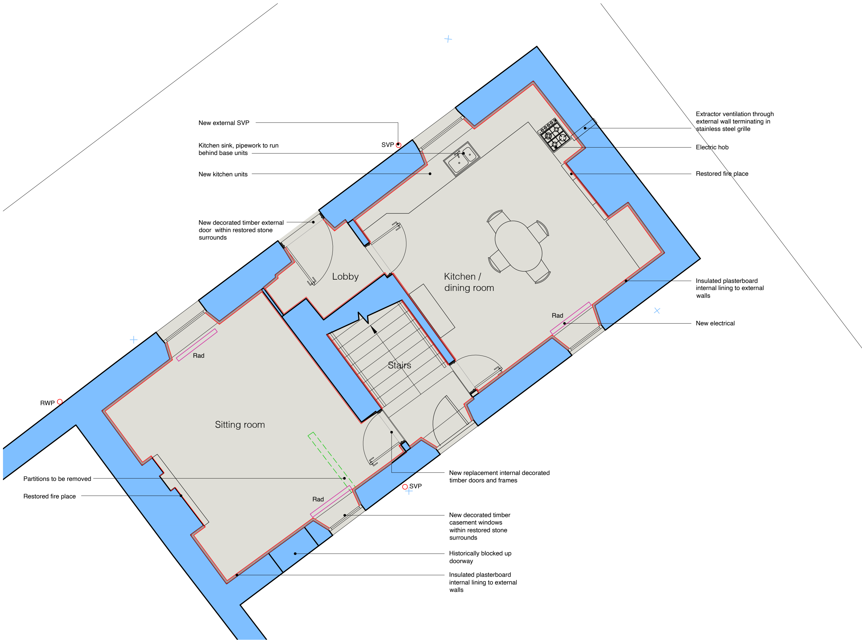
Ground Floor
