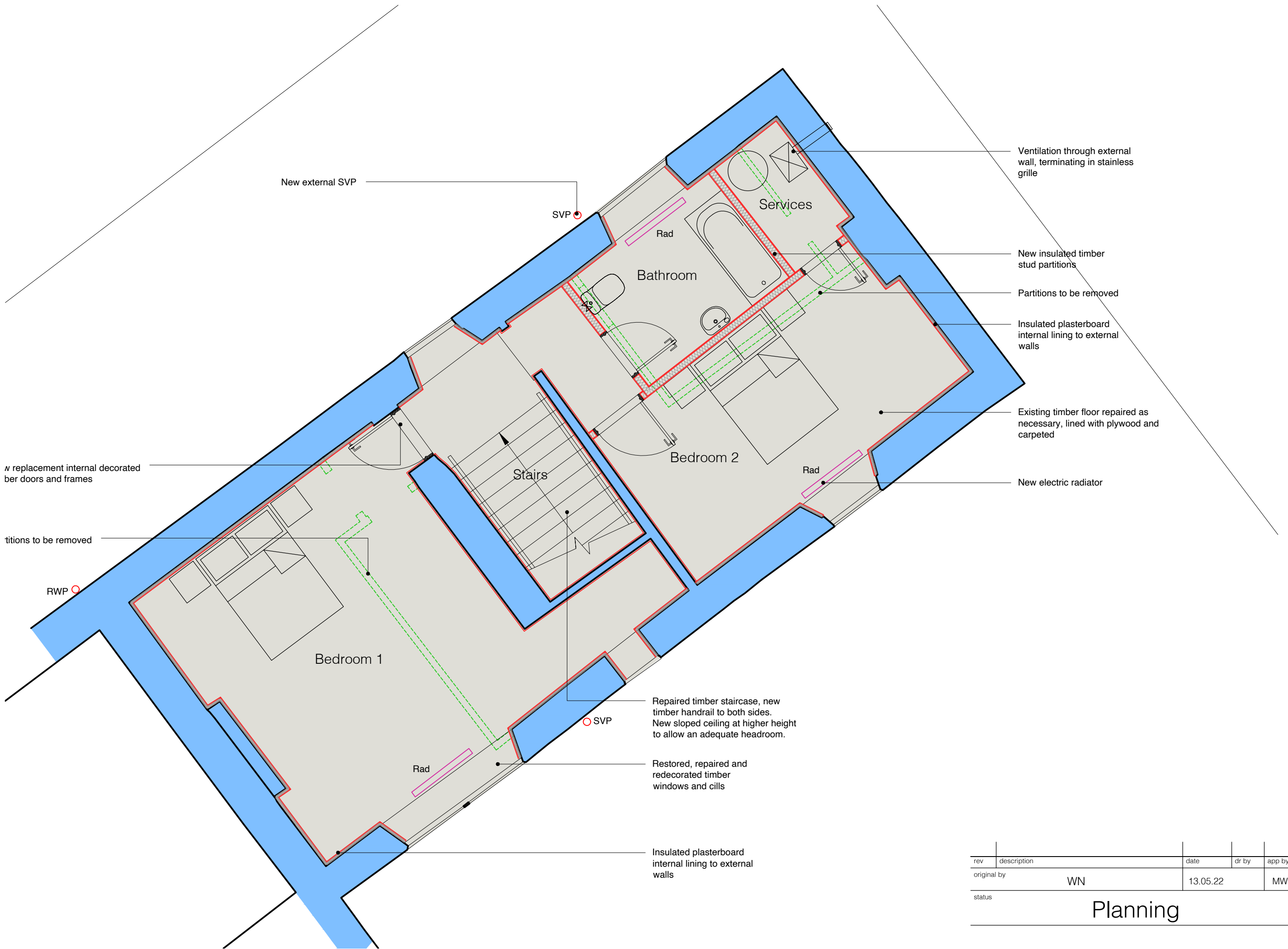
1st. Floor
