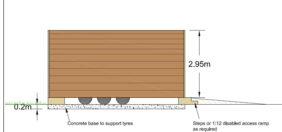
Indicative Side Elevation
