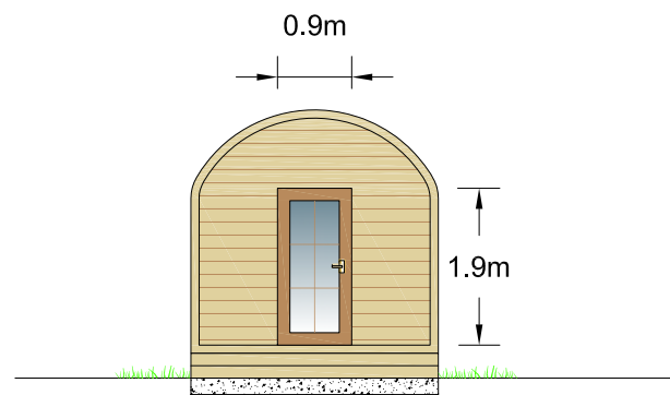
Indicative Front Elevation
