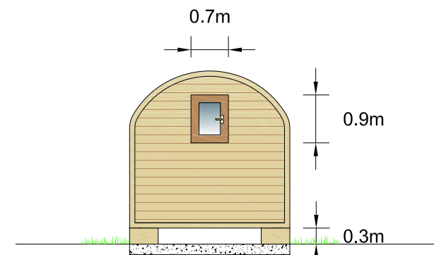
Indicative Rear Elevation
