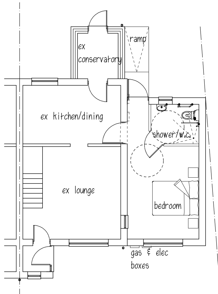
GROUND FLOOR
