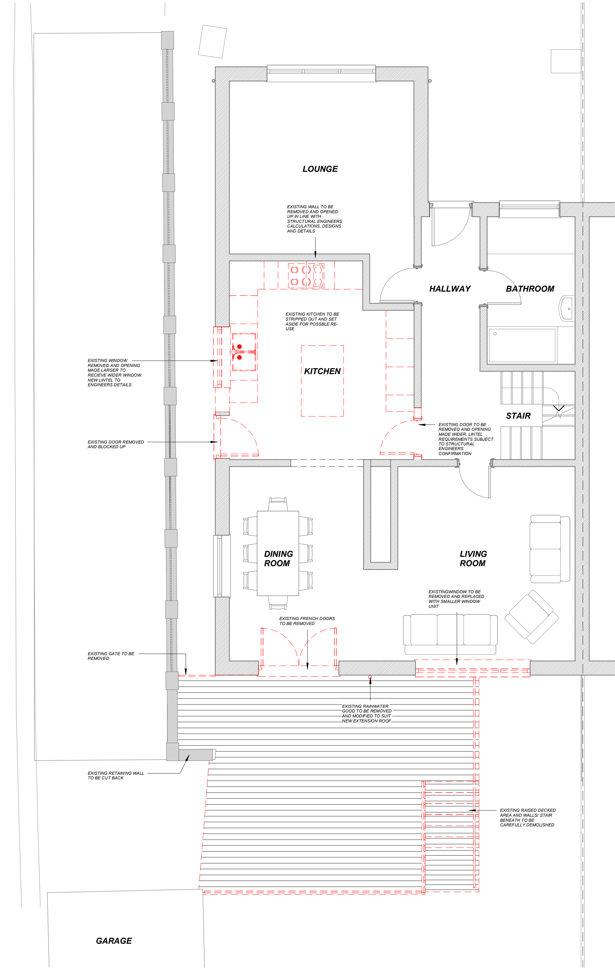
EXISTING GROUND FLOOR GA PLAN 1 : 50
