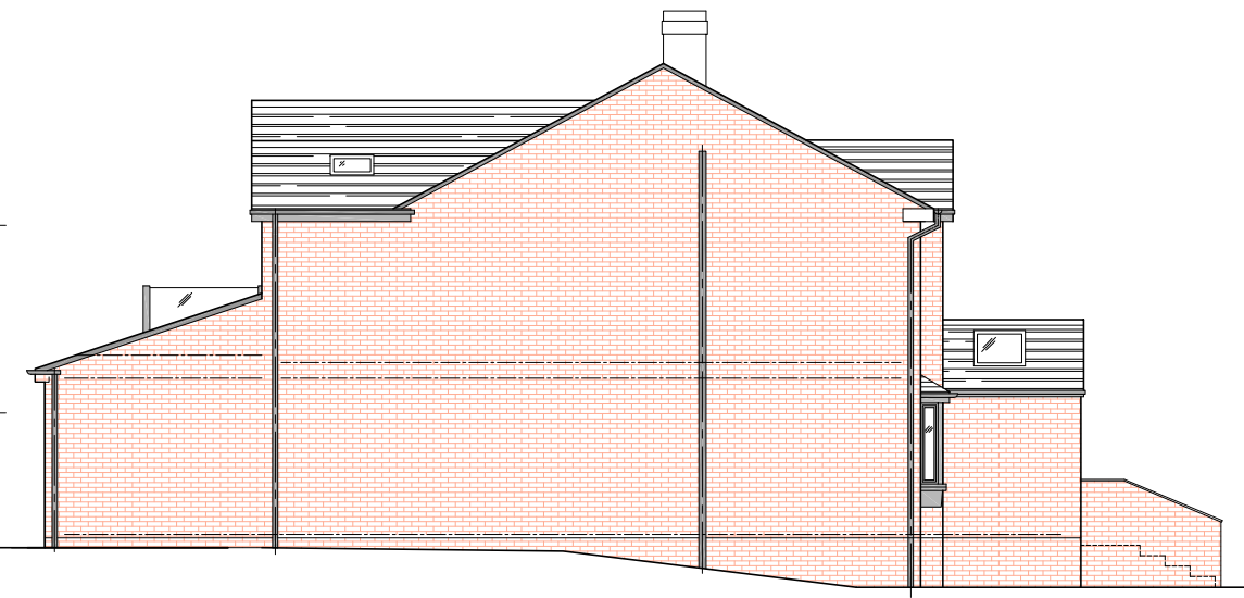
PROPOSED SIDE ELEVATION ON 'B'
