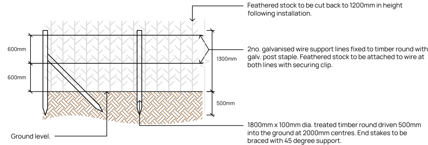
Detail 5 - Typical Feathered Stock Support Detail (N.T.S.)
