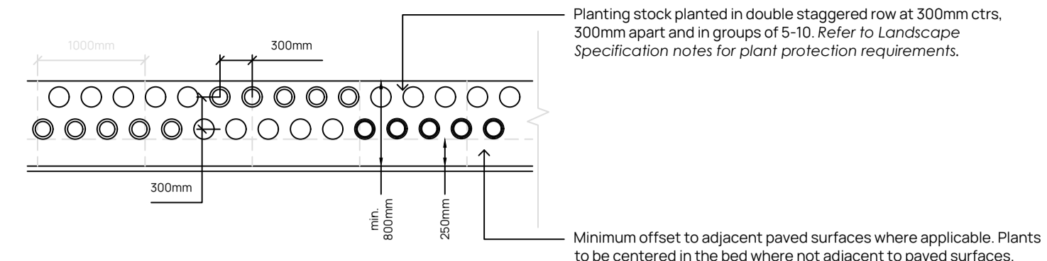
Detail 3 - Typical Native Hedgerow Double Staggered Layout (N.T.S.)
