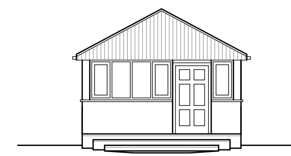
3 NORTH ELEVATION 90-01 1:100
