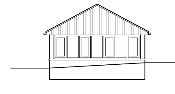
5 SOUTH ELEVATION 90-01 1:100
