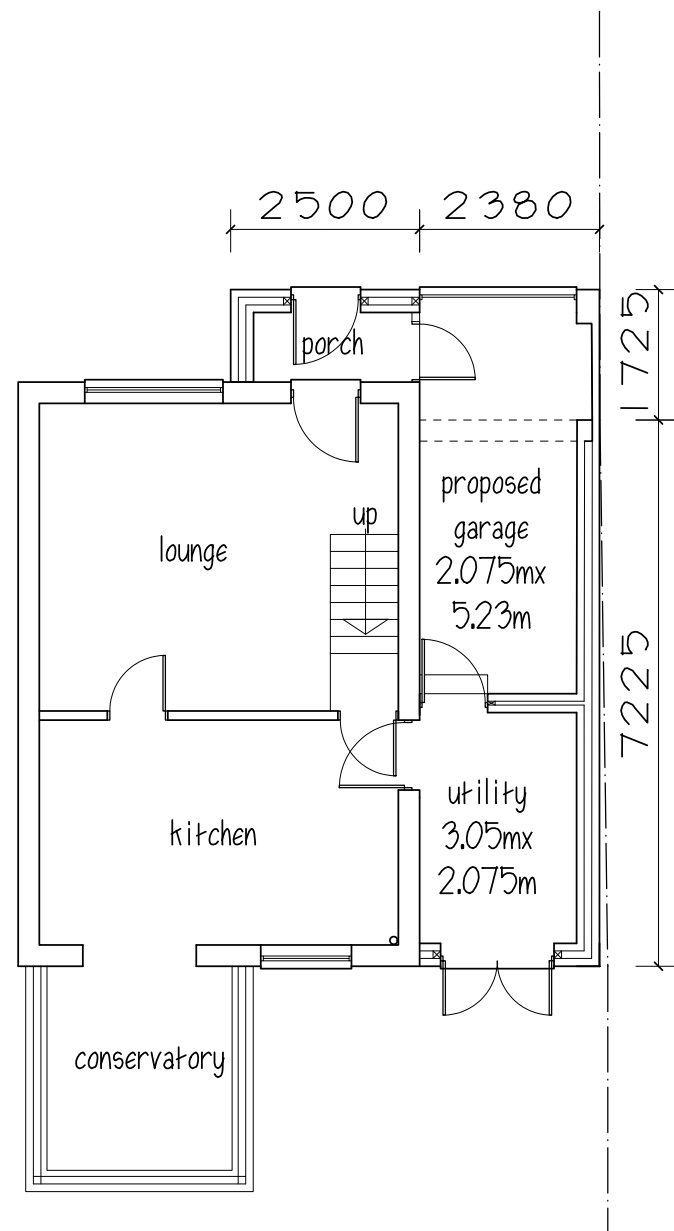
GROUND FLOOR
