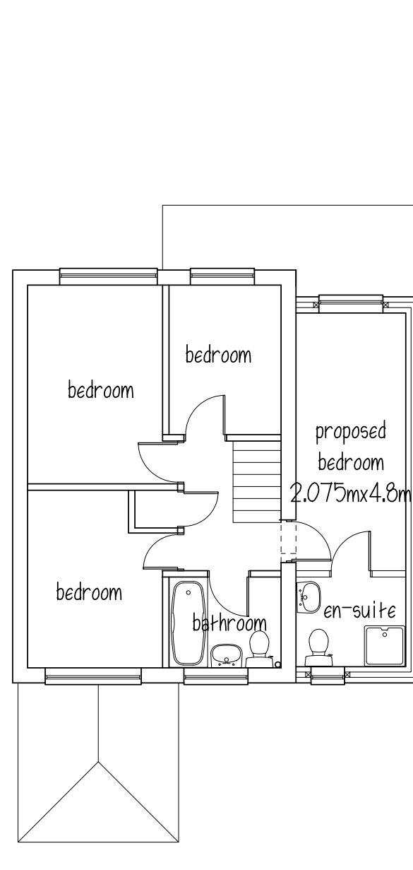
FIRST FLOOR
