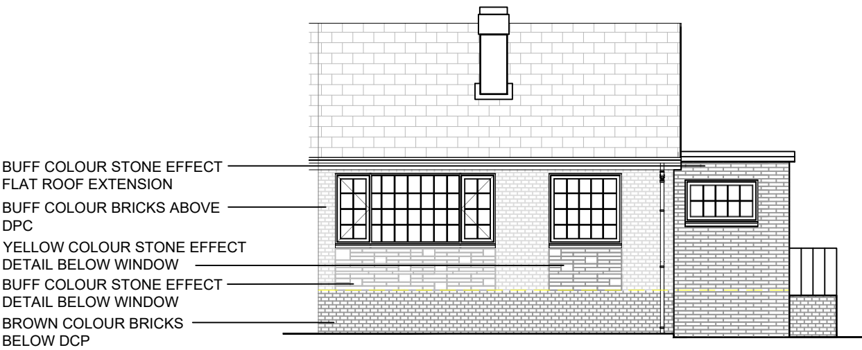
FRONT ELEVATION
