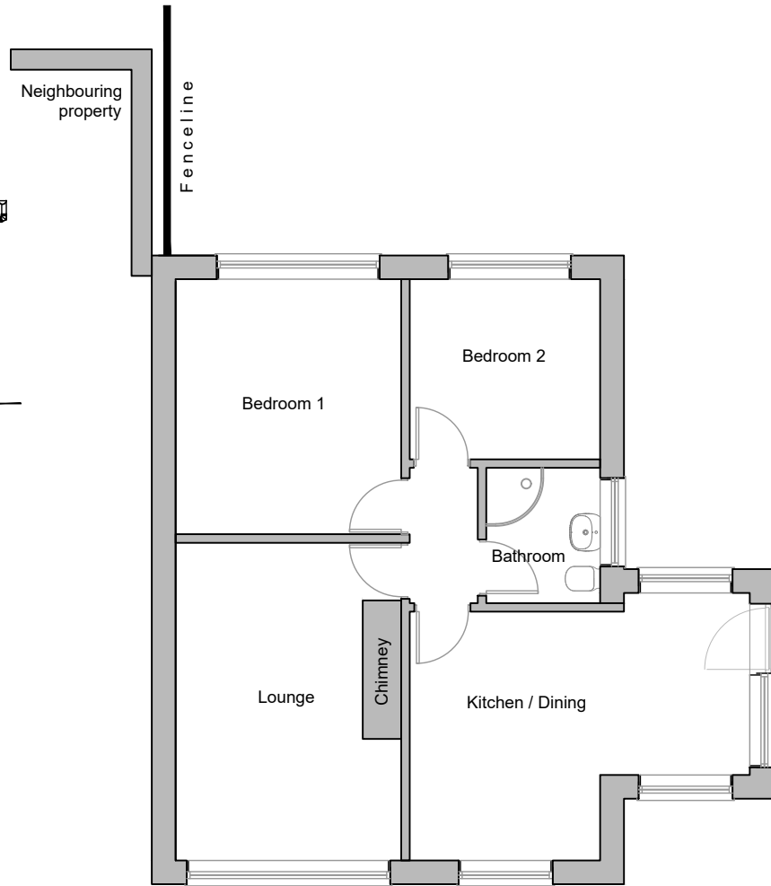
FLOOR PLAN
