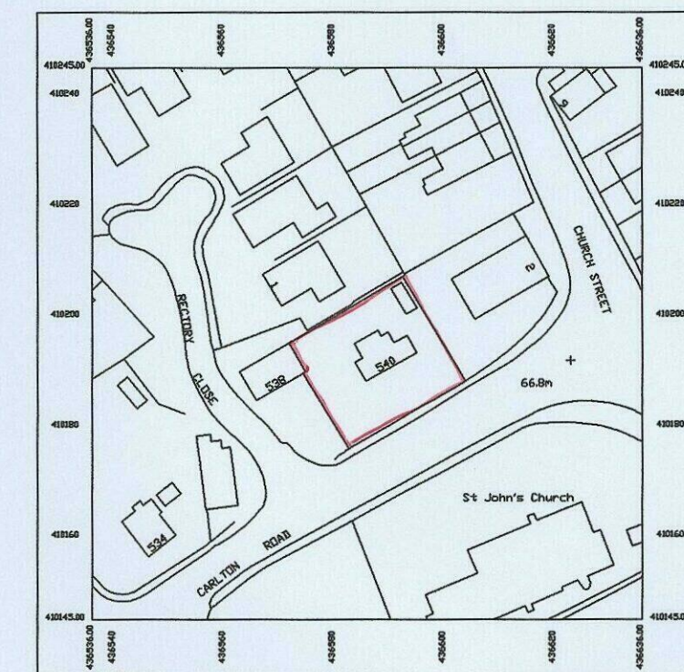
LOCATION PLAN - 1:1250
