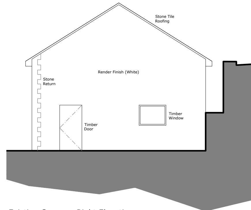
Existing Garage - Right Elevation
