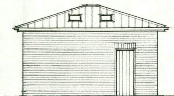
SIDE ELEVATION. 1:100
