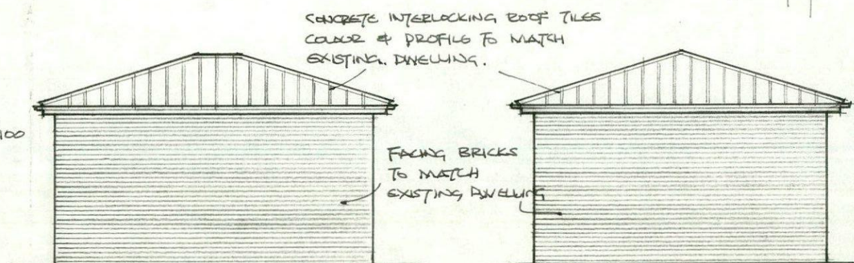
SIDE ELEVATION. 1:100
