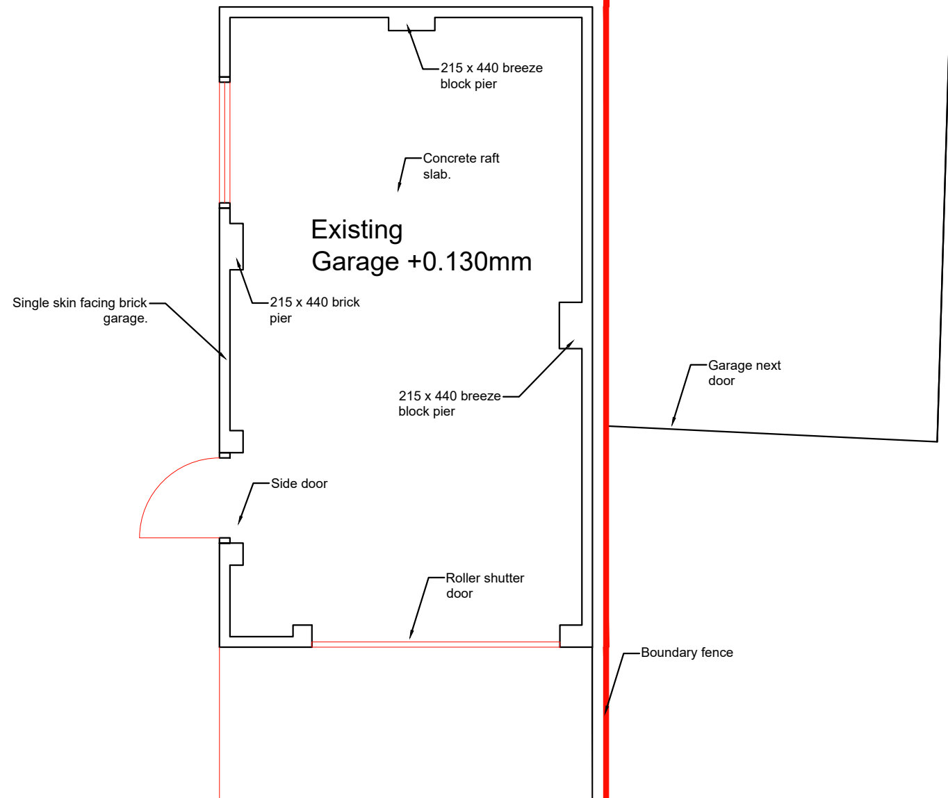
Existing plan 1:50
