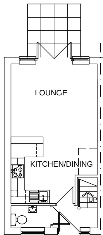
GROUND FLOOR PLAN FIRST FLOOR PLAN HOUSE TYPE A
