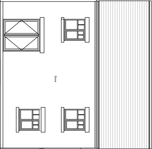
Rear Elevation 1:100
