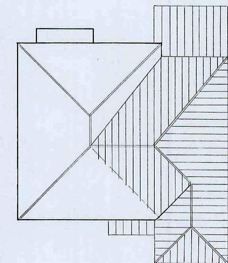
ROOF PLAN
