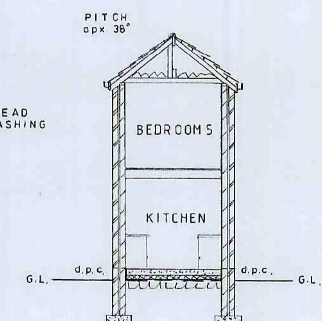
SECTION
