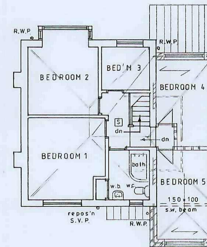
PROPOSED F.F. PLAN
