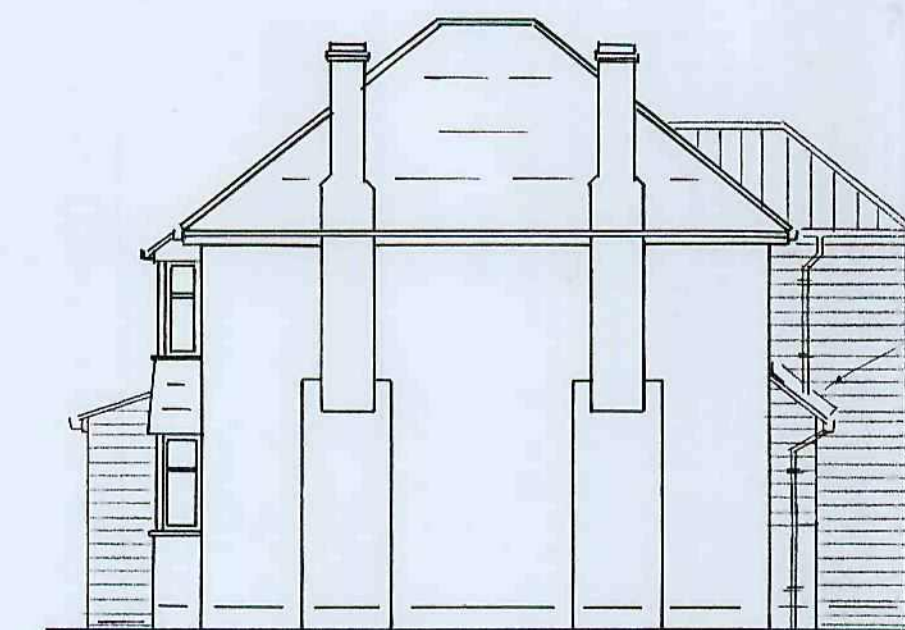
PROPOSED SIDE NORTH
