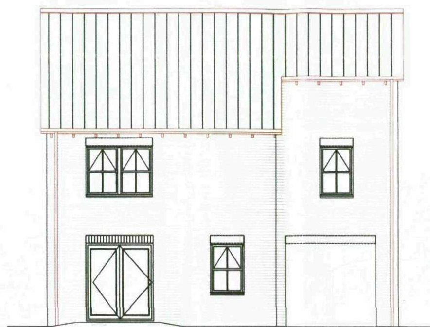
REAR ELEVATION
