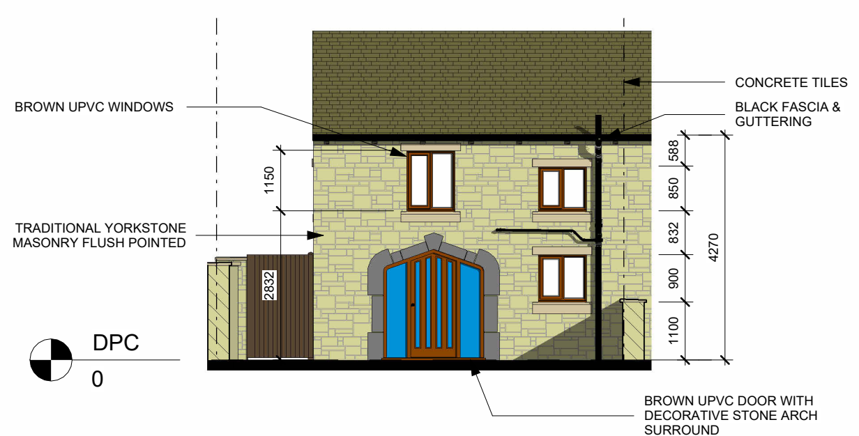
Rear Elevation 1 : 100
