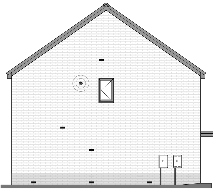
LEFT ELEVATION
