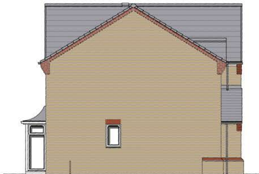
Side Elevation
