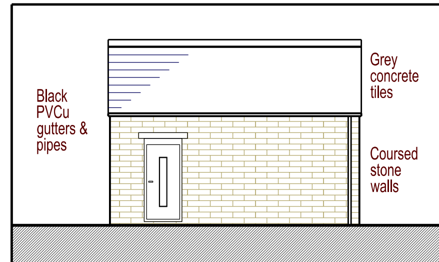
Garage North Elevation - Proposed
