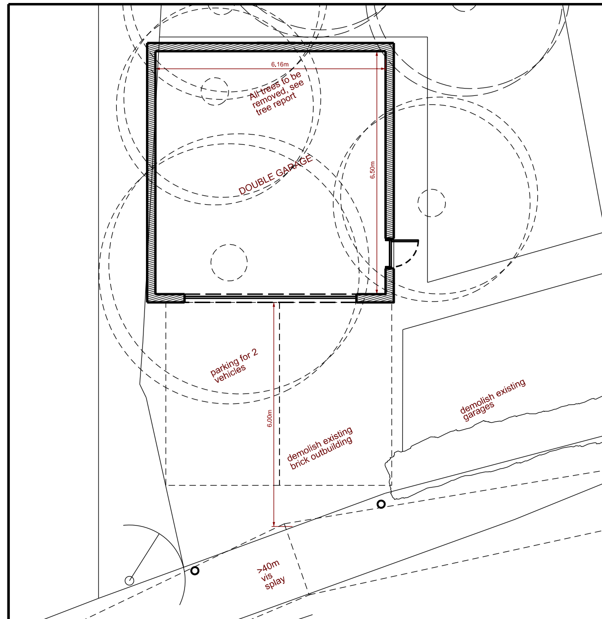
Garage Plan - Proposed
