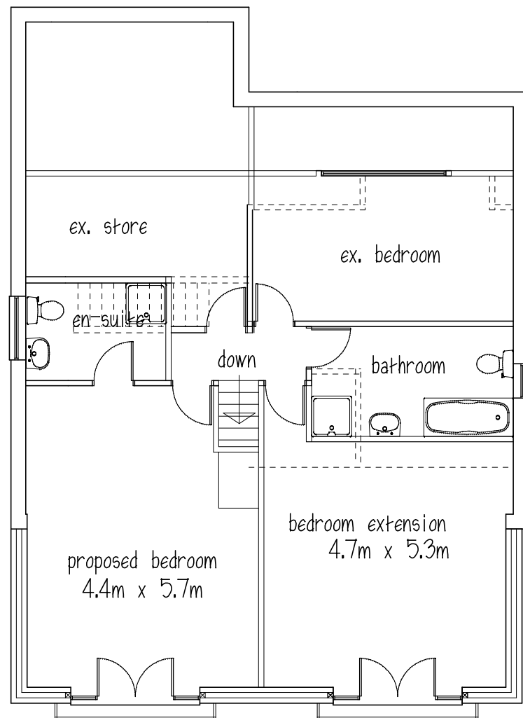
FIRST FLOOR
